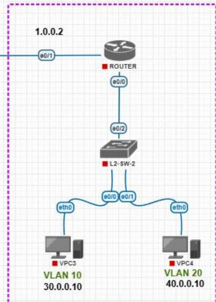
ROUTER ON-A-STICK
